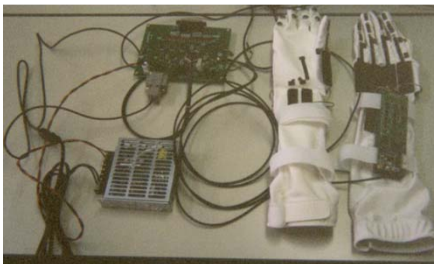
Figure 9. Prototype of StrinGlove.
